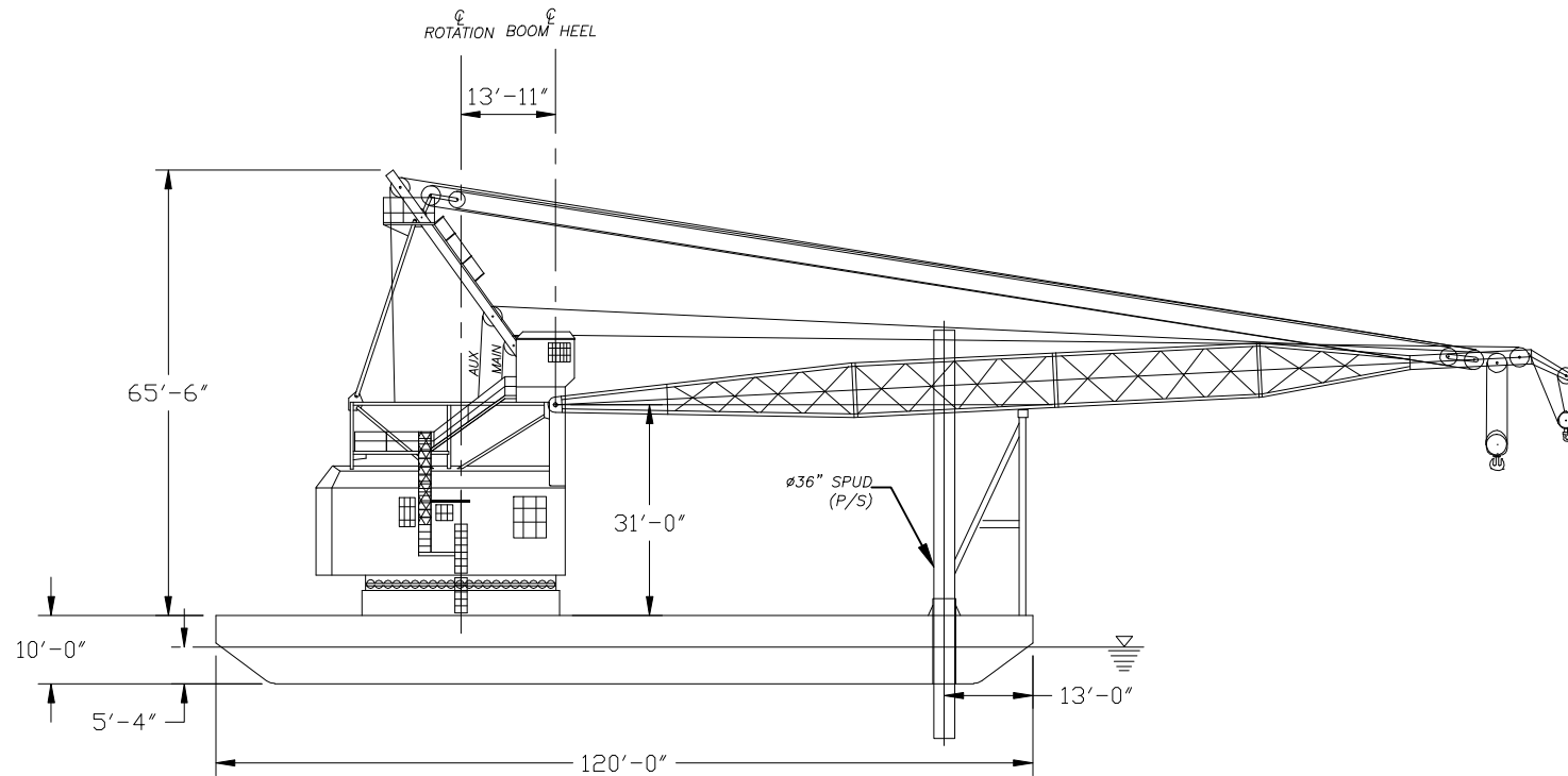
OUTBOARD PROFILE
